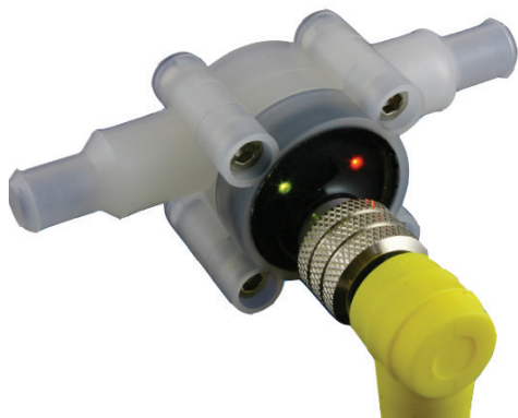
PNP-NPN version with M12 connector
